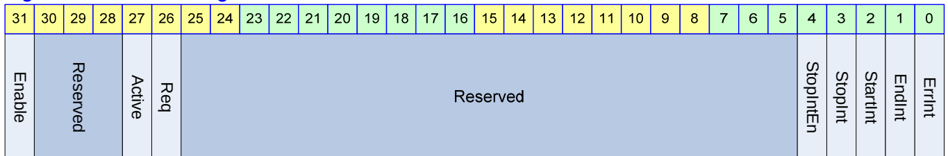
Figure 9-8 Status Register
