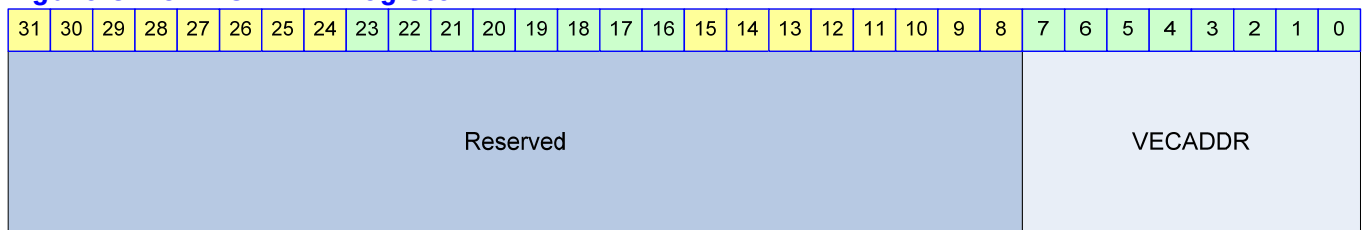
Figure 8-15 VECADDR Register
