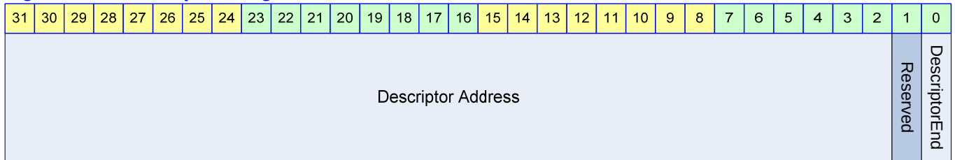
Figure 9-7 Descriptor Register
