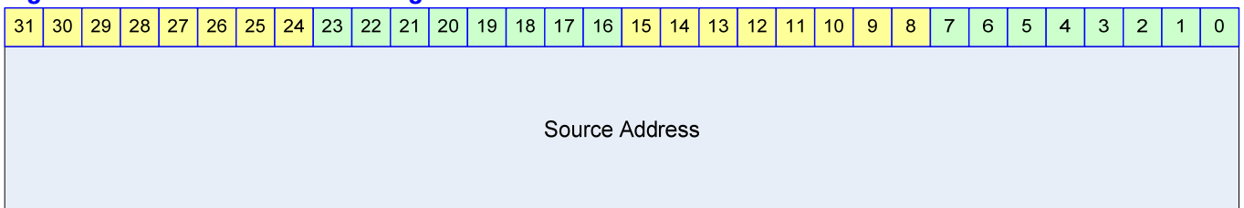
Figure 9-4 Source Address Register
