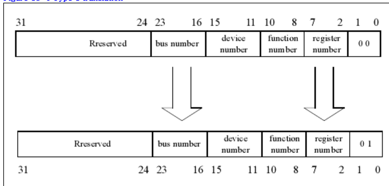
Figure 18-4 Type 1 translation
