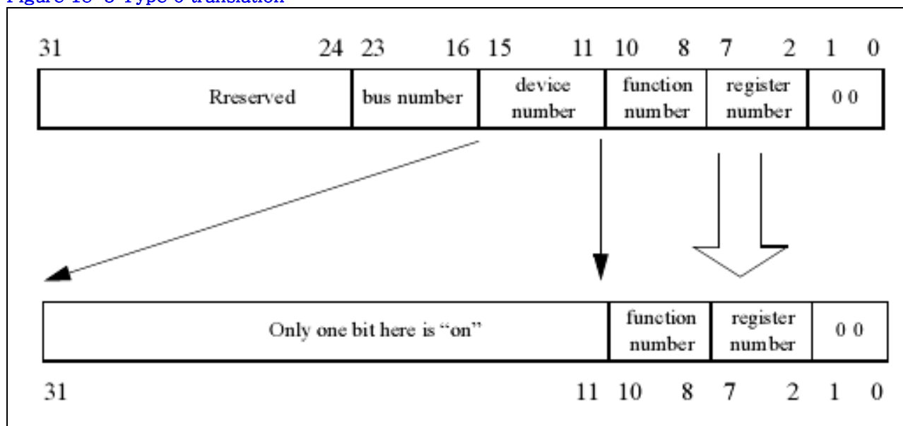
Figure 18-3 Type 0 translation
