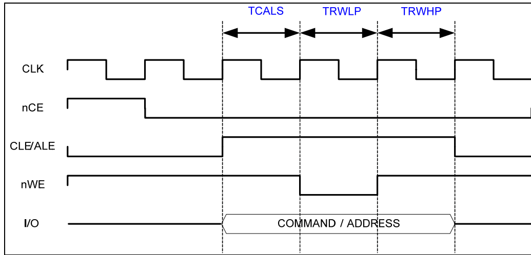
Figure 17-3 ALE,CLE Timing
